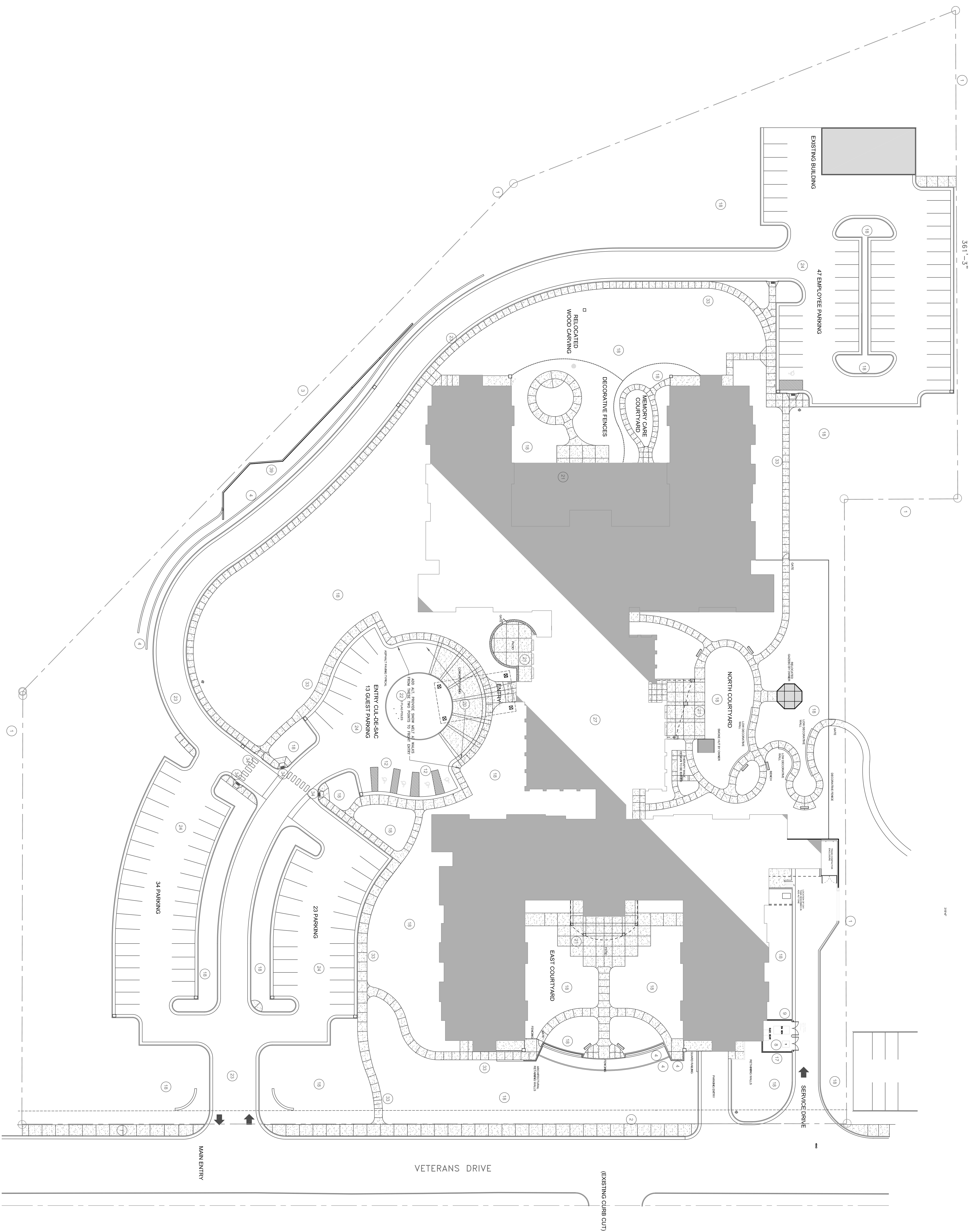
ARCHITECTURAL SITE PLAN SCALE: 1" = 30'-0"
