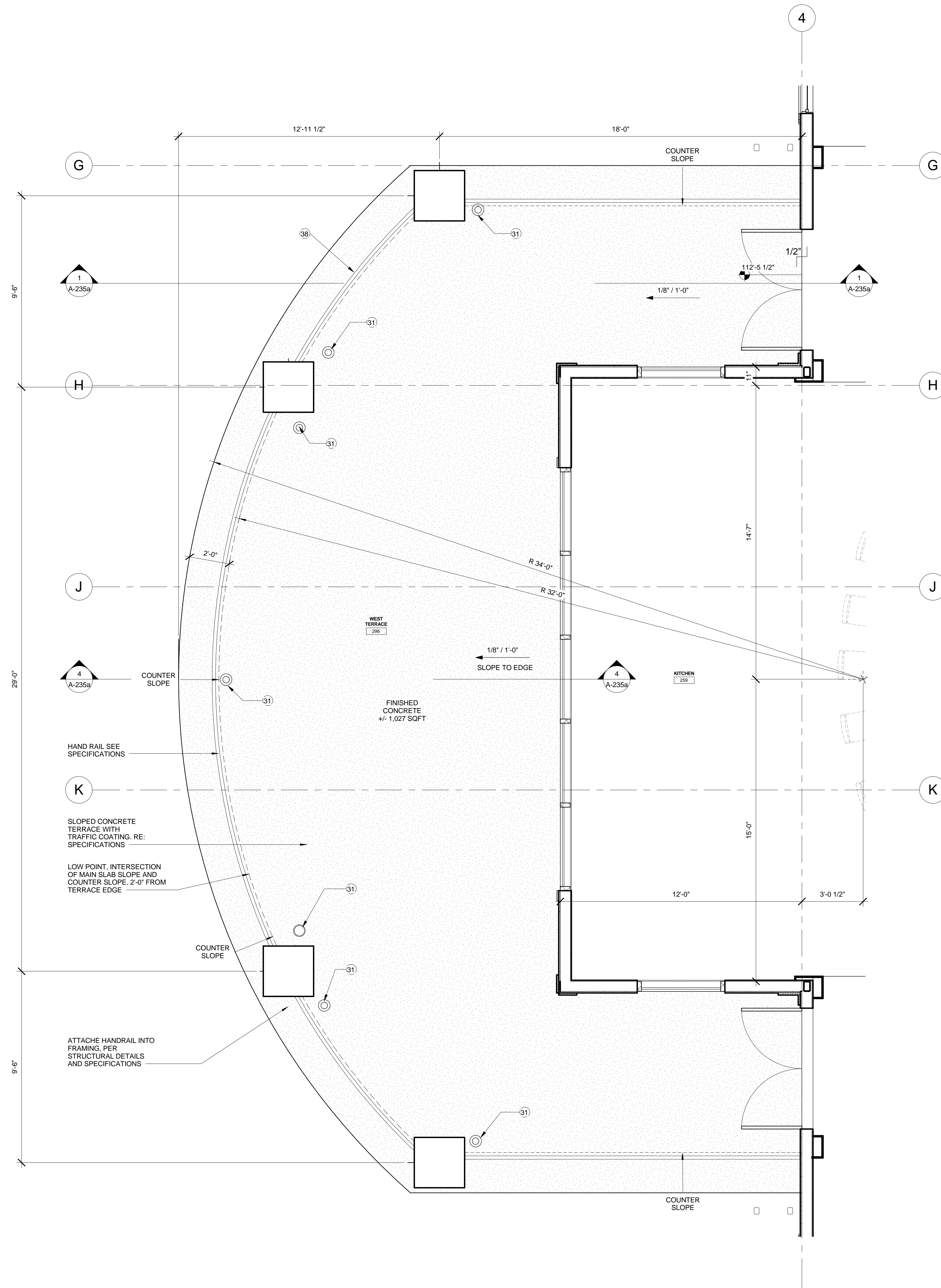
1 TERRACE AT ZONE 1 & 2 SCALE: 3/8" = 1'-0"
