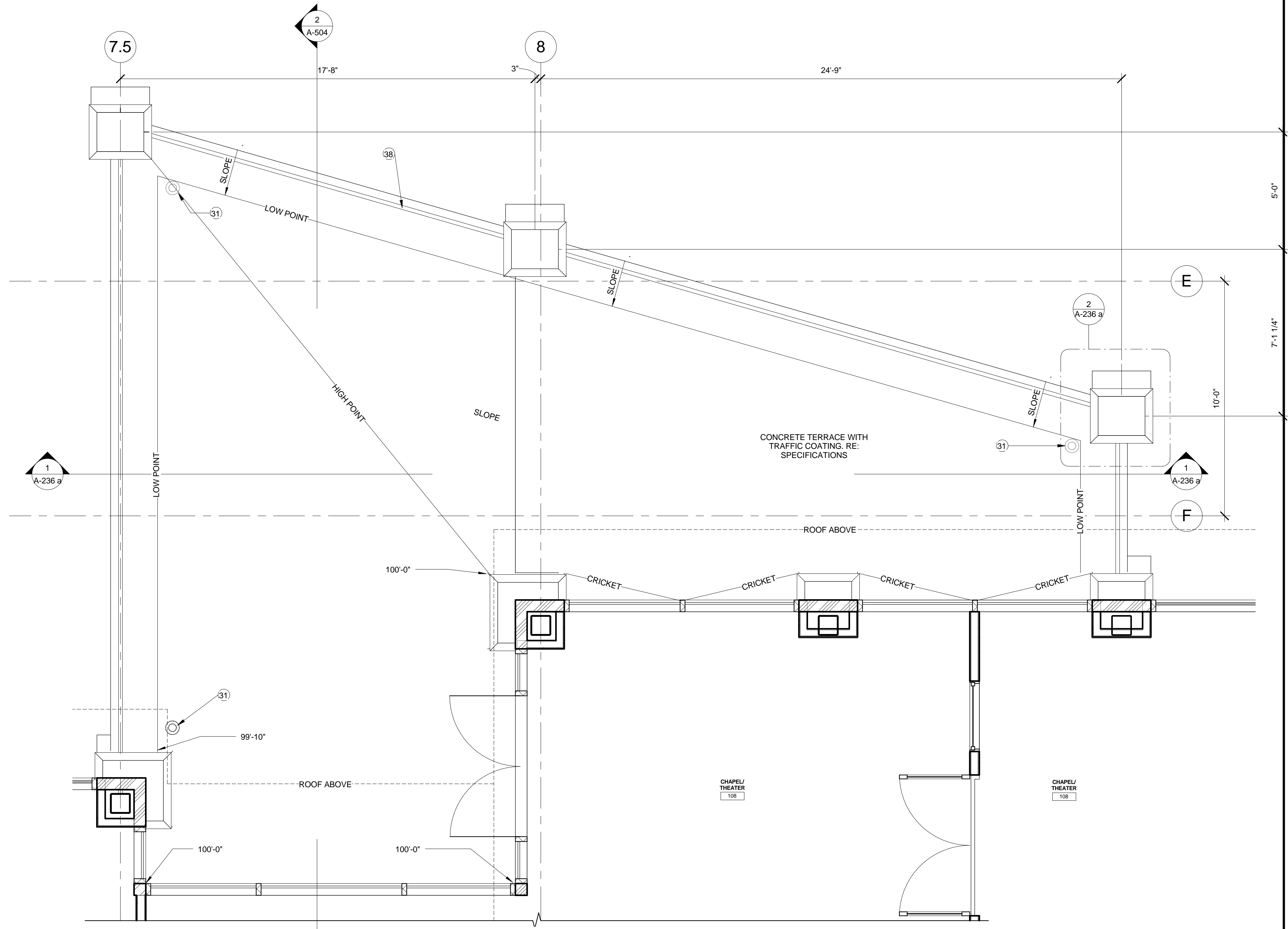
1 TERRACE AT TOWN CENTER SCALE: 3/8" = 1'-0"
