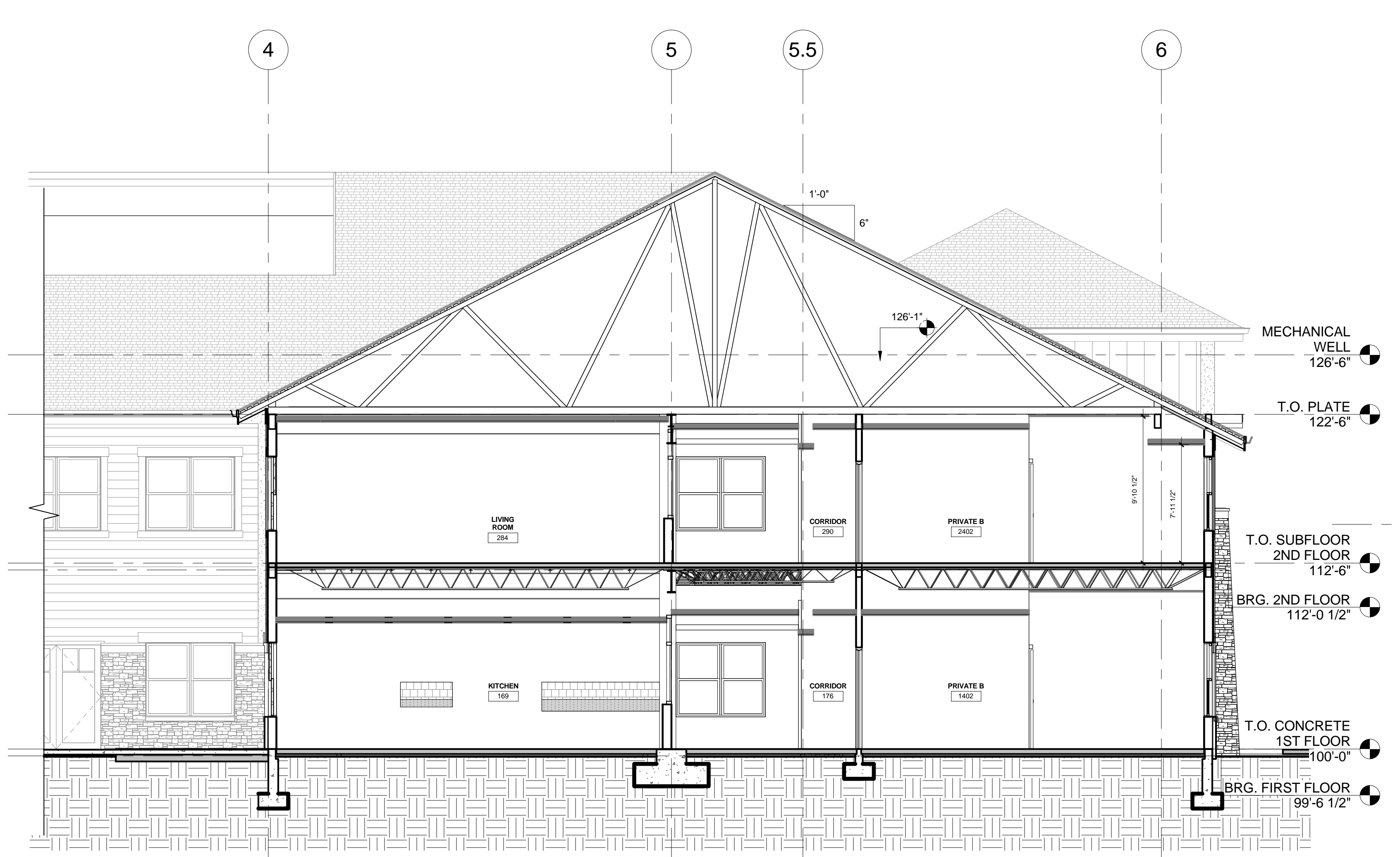
D BLDG. SECTION D SCALE: 3/16" = 1'-0"
