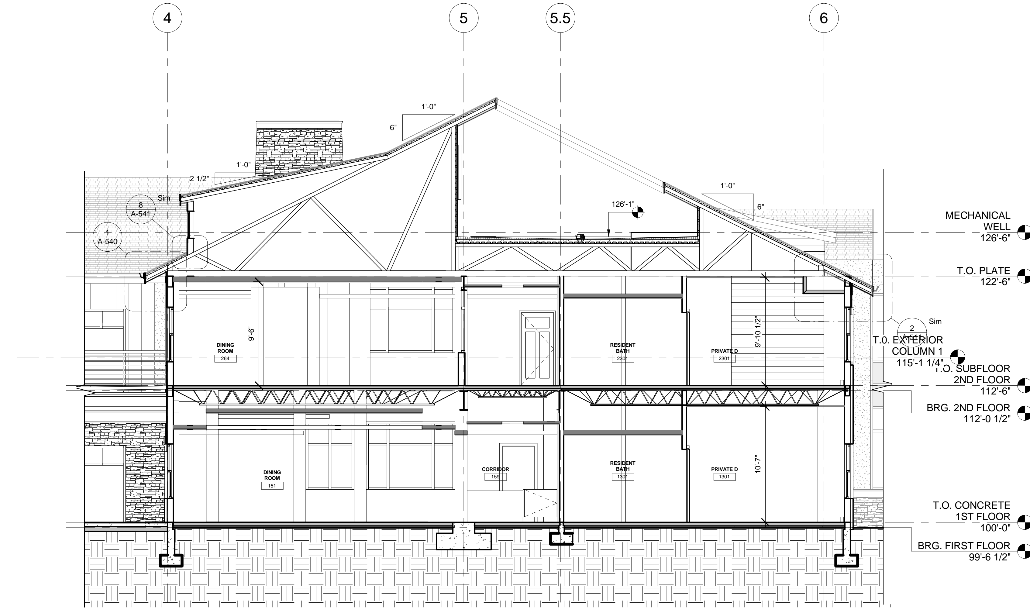
C BLDG. SECTION C SCALE: 3/16" = 1'-0"
