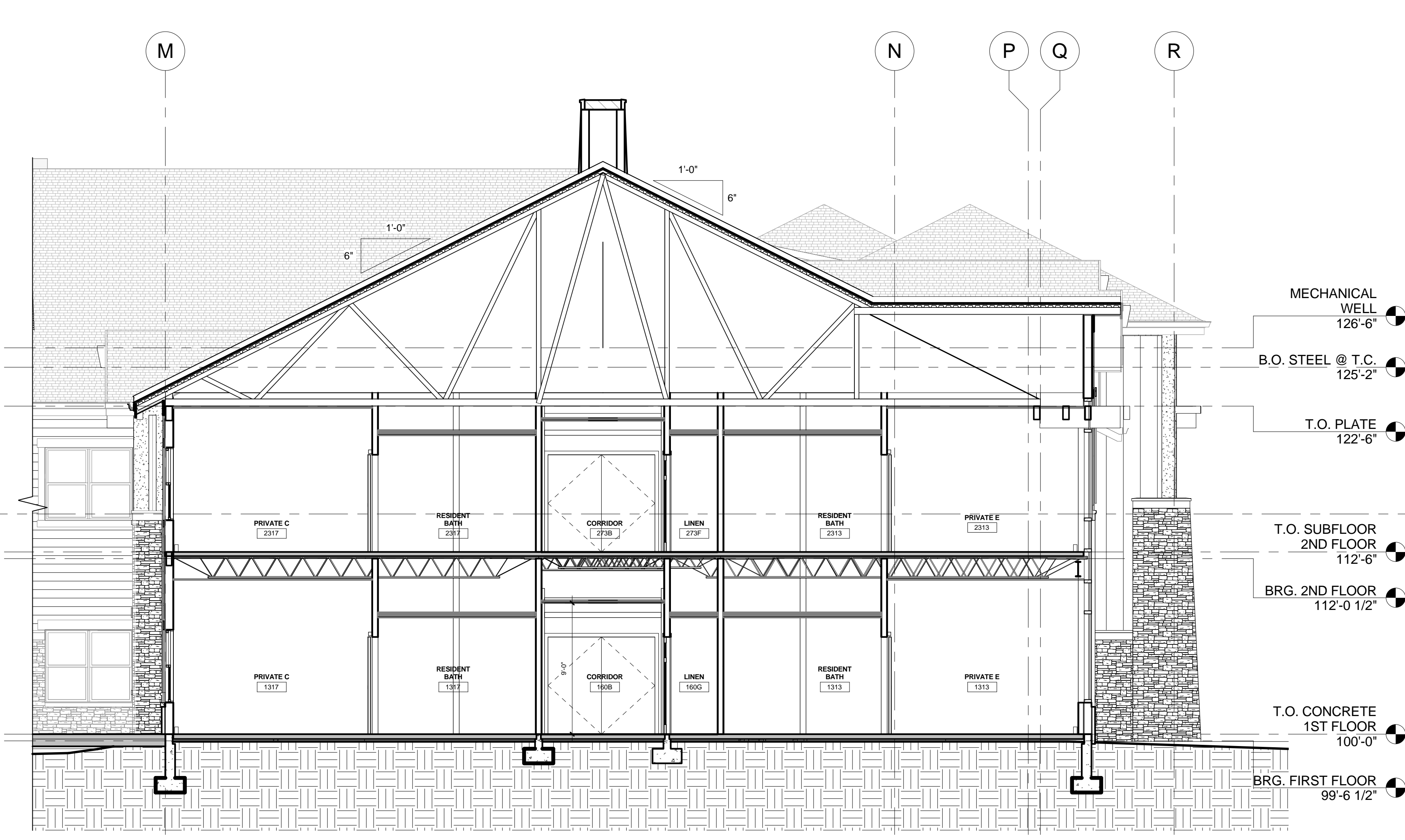
B BLDG. SECTION B SCALE: 3/16" = 1'-0"
