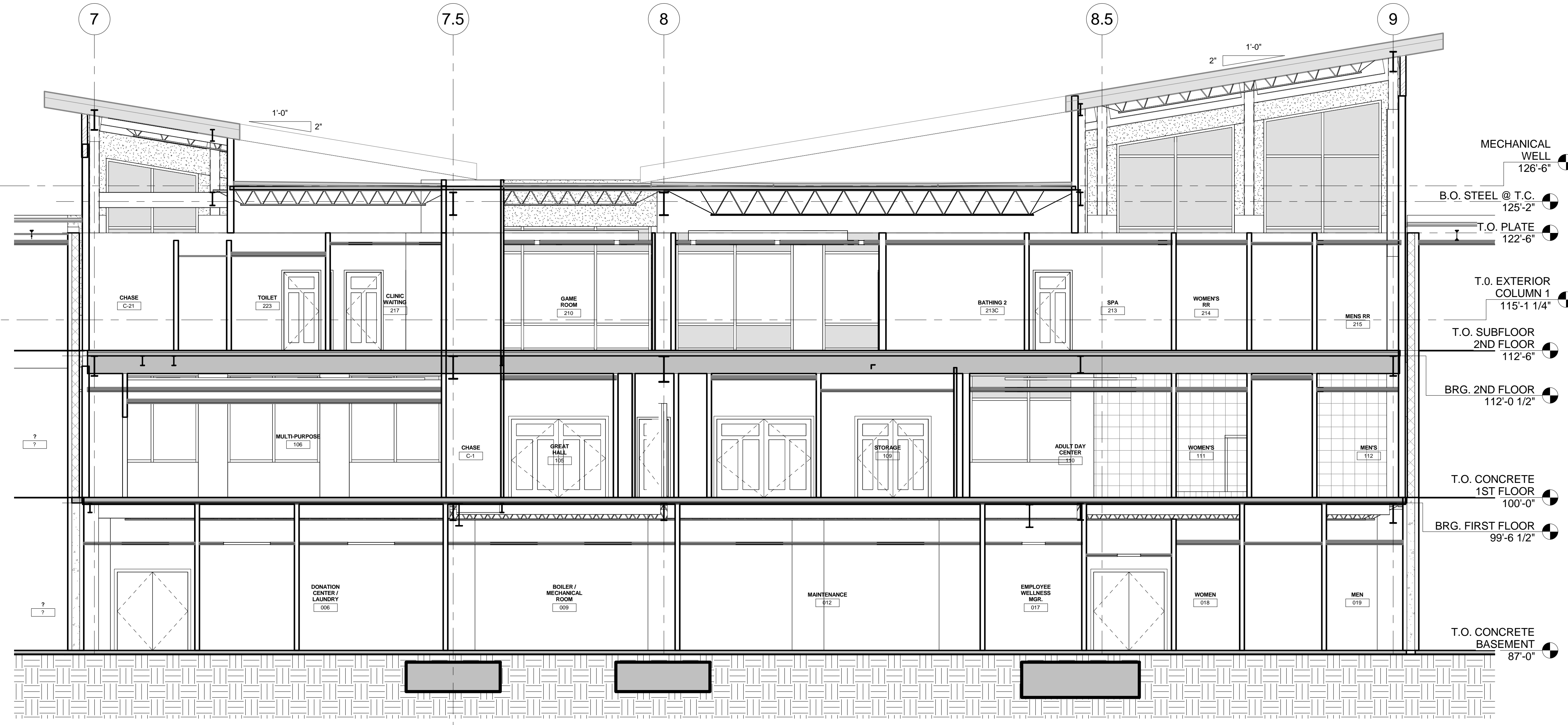
1 ZONE 3, SECTION THRU ROOF ACCESS SCALE: 3/16" = 1'-0"
